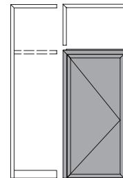
Wechselprofil-Bauweise Reverse rebate profile construction method
